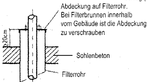
Detail Brunnenkopf
